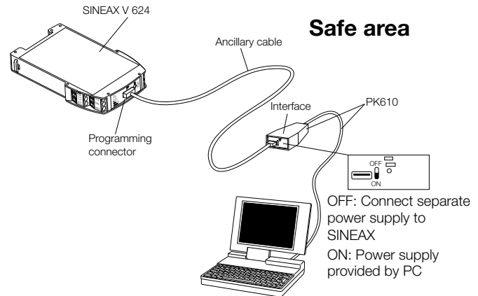
Fig. 2. Example of the set-up for programming a SINEAX V624 in standard version without the power supply. For this case the switch on the interface must be set to "ON".
