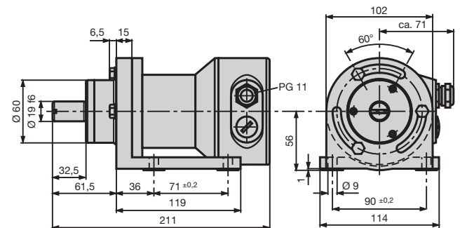
Fig 5. KINAX WT717 with additional gear and foot.
