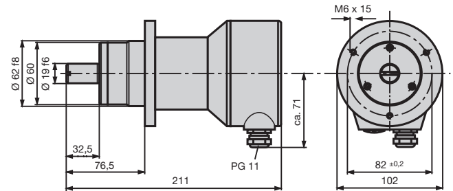
Fig 4. KINAX WT717 with additional gear.
